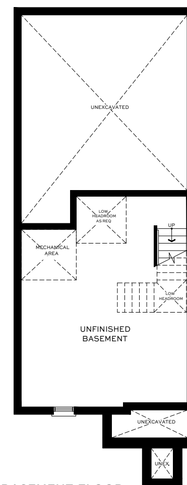
BASEMENT FLOOR ELEV. A1/A2
