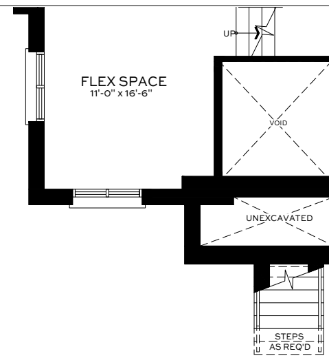
GROUND FLOOR ELEV. B1
