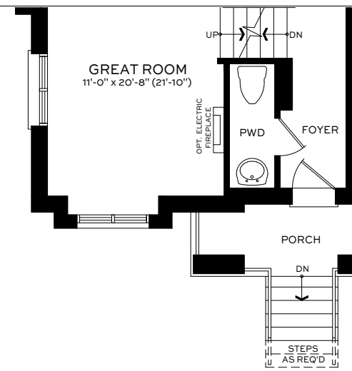
MAIN FLOOR ELEV. B1
