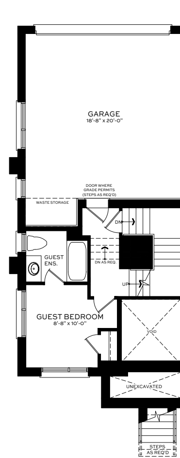
OPT. GROUND FLOOR ELEV. A1
