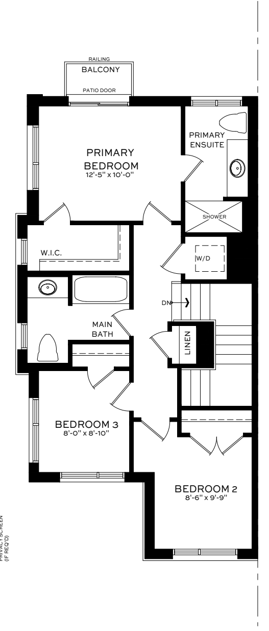
UPPER FLOOR ELEV. A1
