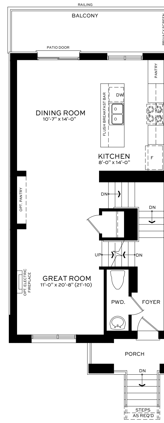
MAIN FLOOR ELEV. A1
