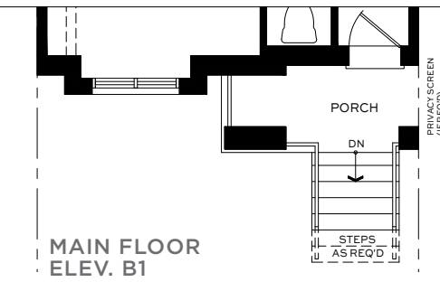
MAIN FLOOR ELEV. B1
