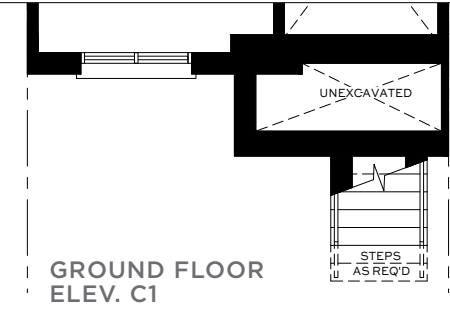
GROUND FLOOR ELEV. C1
