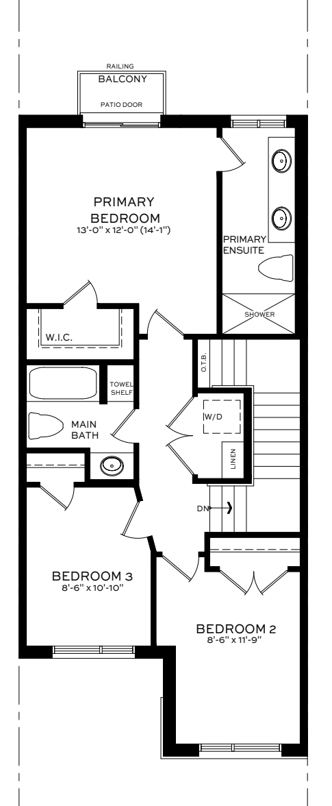
UPPER FLOOR ELEV. A1
